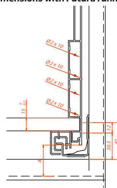
Dimensions with Futura runners
