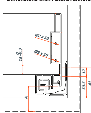
Dimensions with Futura runners
