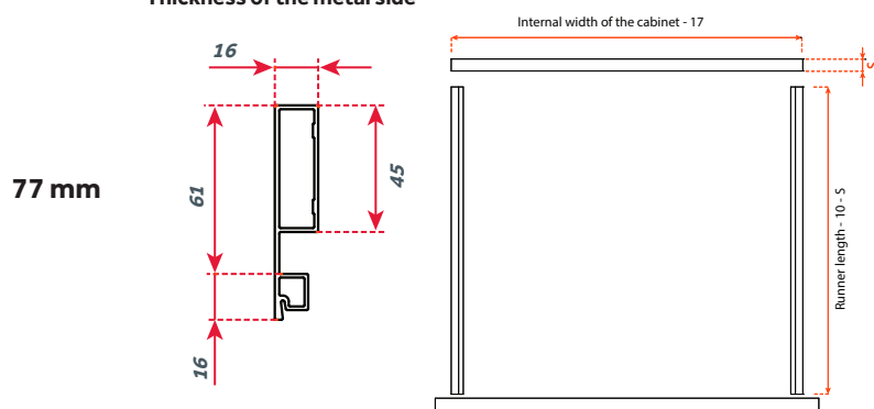
Thickness of the metal side
